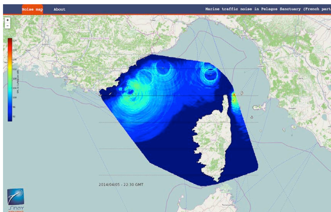
Figure 5. Online map of noise according to a model fed in real-time by ships tracked with AIS (Automatic Identification System) ( www.oceannoisemap.com )
