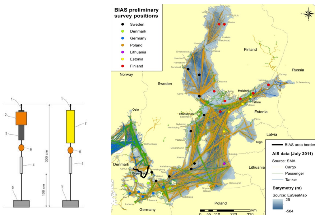
Figure 1. Left: Rig design for the two different recorders used. Legend: 1) hydrophone, 2) flotation (urethane foam), 3) DSG-Ocean, 4) Acoustic releaser, 5) disposable anchor, 6) secondary flotation and 7) SM2M. Right: Positions of recording stations within the BIAS project plotted on top of a map showing shipping density from AIS data
